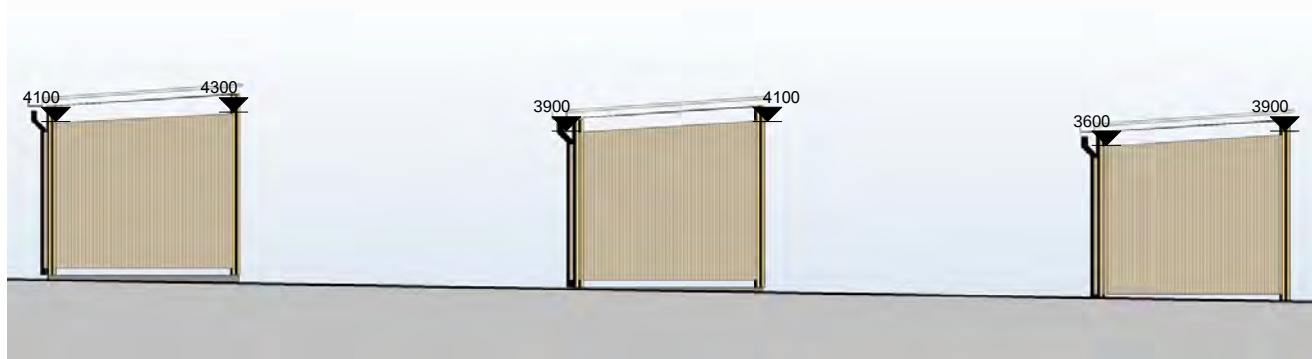
Figure 35 Bus shelter elevations and visualisation
